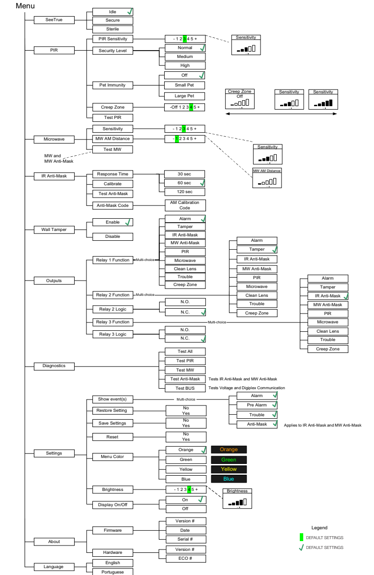
Figure 6: NVX80 Menu Tree
