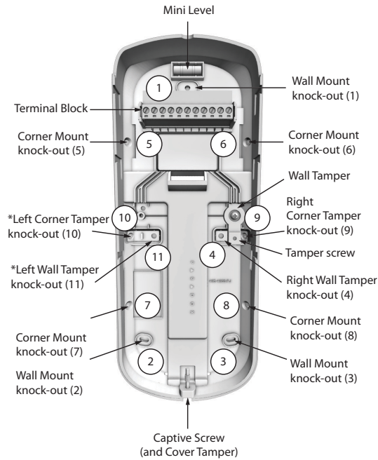
Figure 2: NVX80 Back Cover Components
