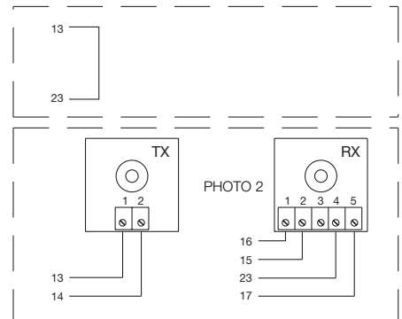
Fig. 3C Shows how to connect Phototest with just the Photo 2 photocell
