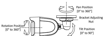
Figure 2-3 3-Axis Adjustment
