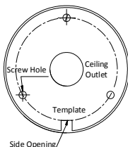
Figure 2-8 Drill Template
