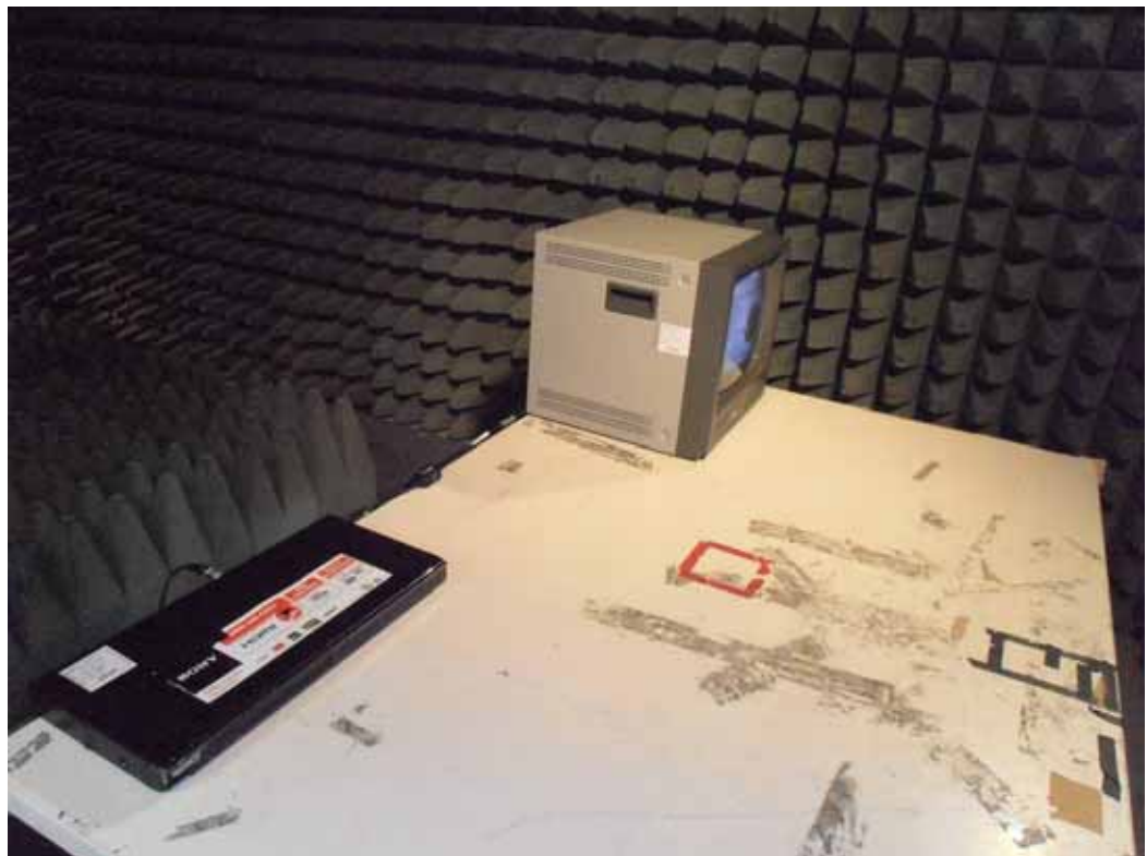
Rear View
