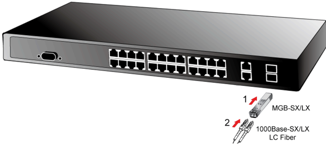
Figure 2-7: Plug-in the SFP transceiver
