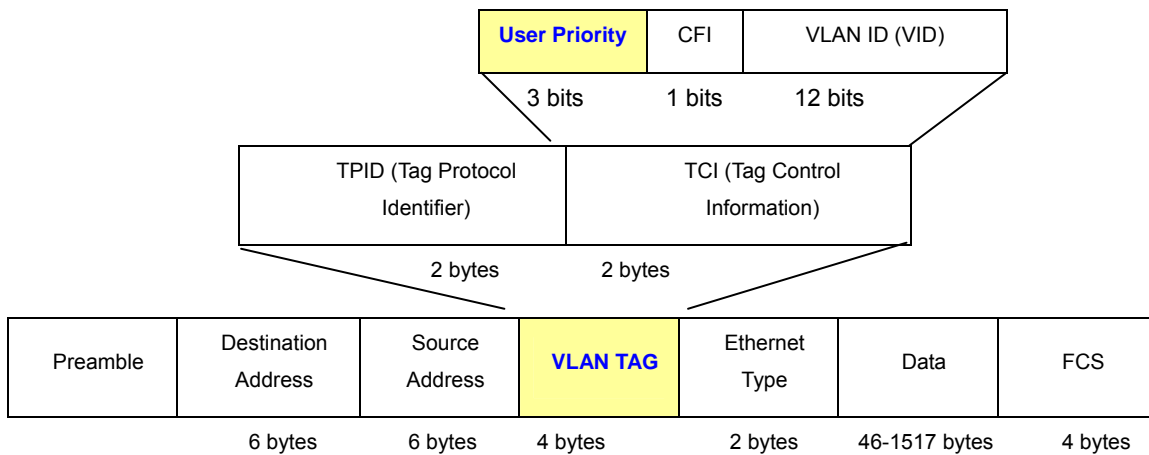
Figure 4-15-1: 802.1p Tag Priority
