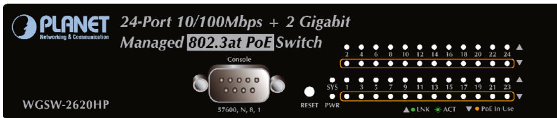
Figure 2-2: WGSW-2620HP LED Panel
