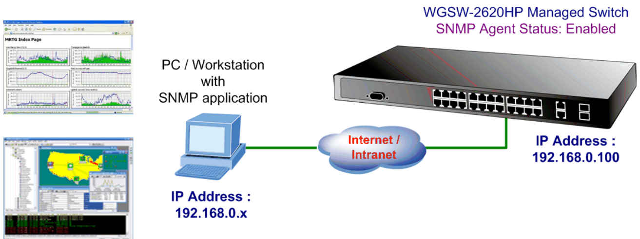
Figure 3-3: SNMP Management Diagram
