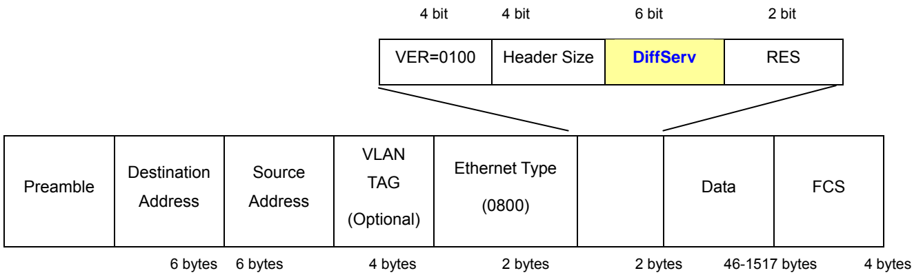
Figure 4-15-4: IPv4 frame format
